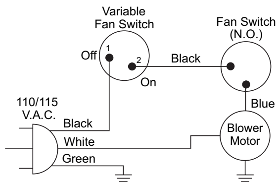
Figure 31 - Fan wire assembly diagram
