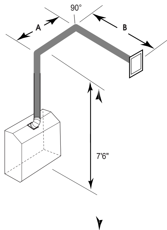
Figure 20 - Horizontal Run Reduction
