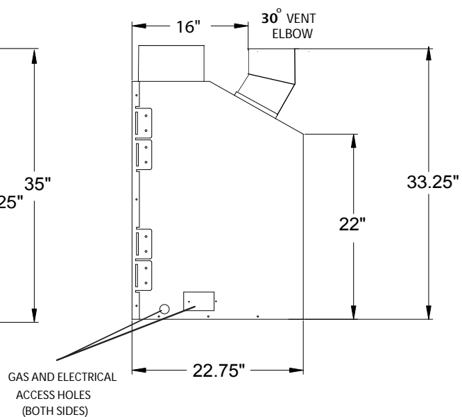
RIGHT SIDE VIEW WITH 30 DEGREE STARTING ELBOW
