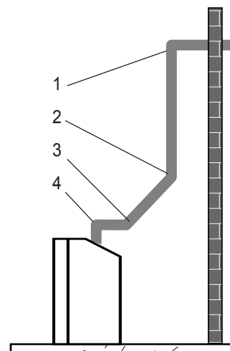
Figure 22 - Maximum Elbow Usage
