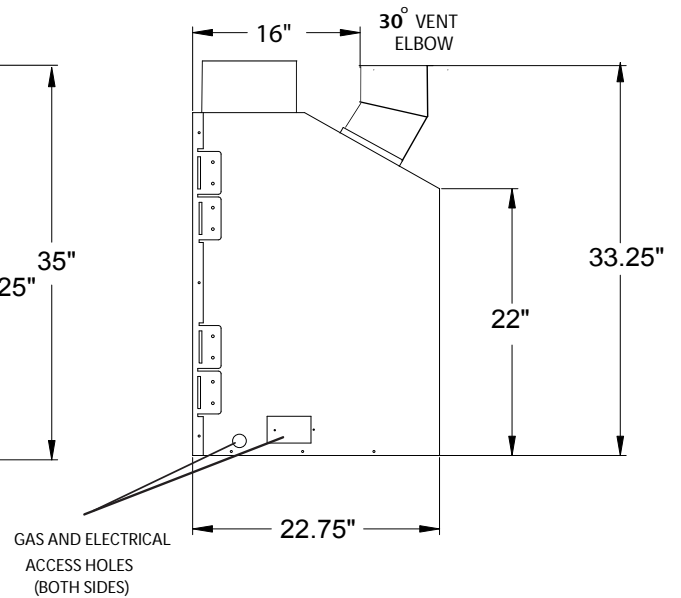
RIGHT SIDE VIEW WITH 30 DEGREE STARTING ELBOW
