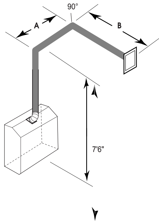
Figure 20 - Horizontal Run Reduction
