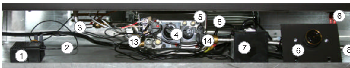
CONTROL COMPARTMENT
