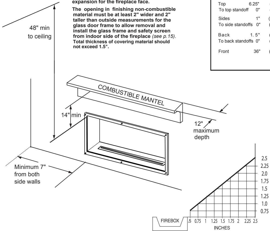
*Minimum 7 inches from Side Wall to Fireplace opening
